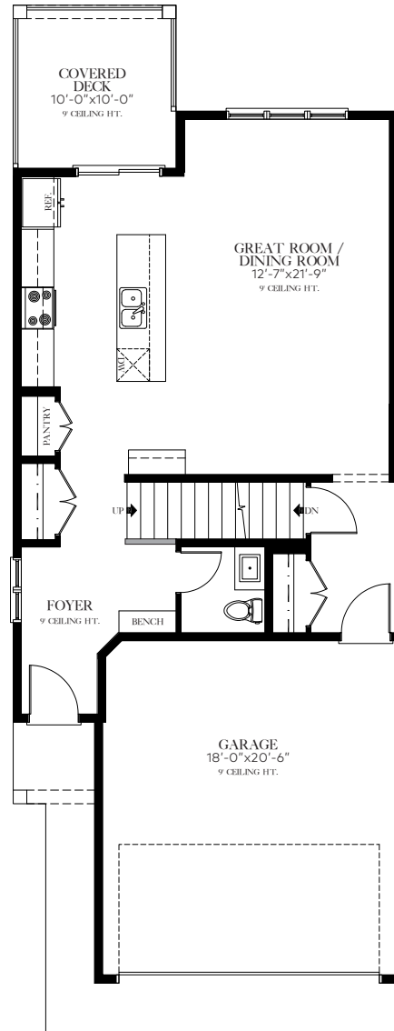
MAIN FLOOR PLAN 774 SQ. FT.
