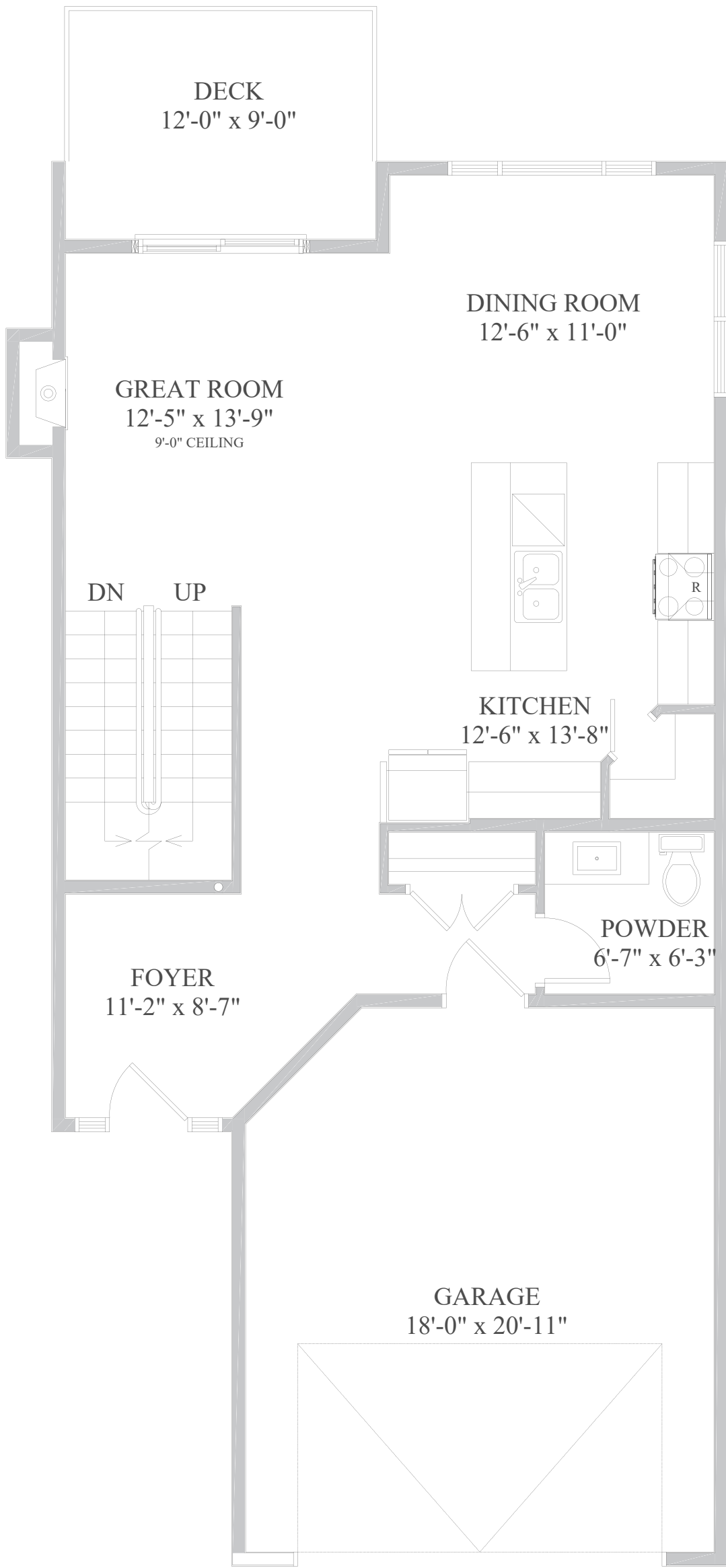
MAIN FLOOR PLAN 772 SQ. FT. + DOUBLE GARAGE
