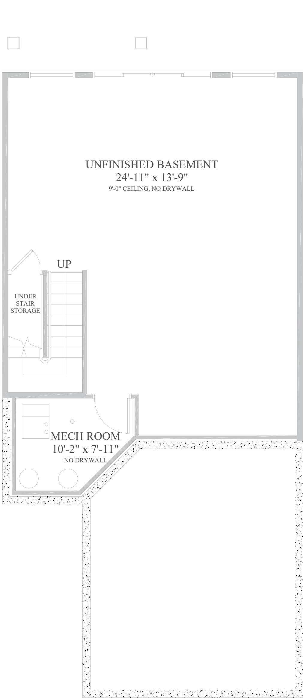
LOWER FLOOR (UNFINISHED OPTION) 817 SQ. FT.
