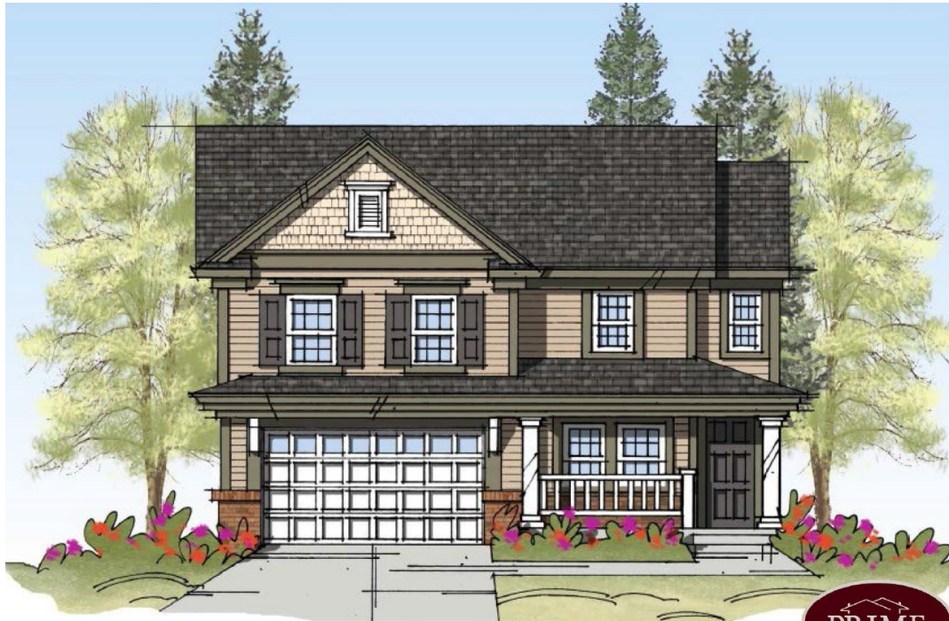
Williams Model
