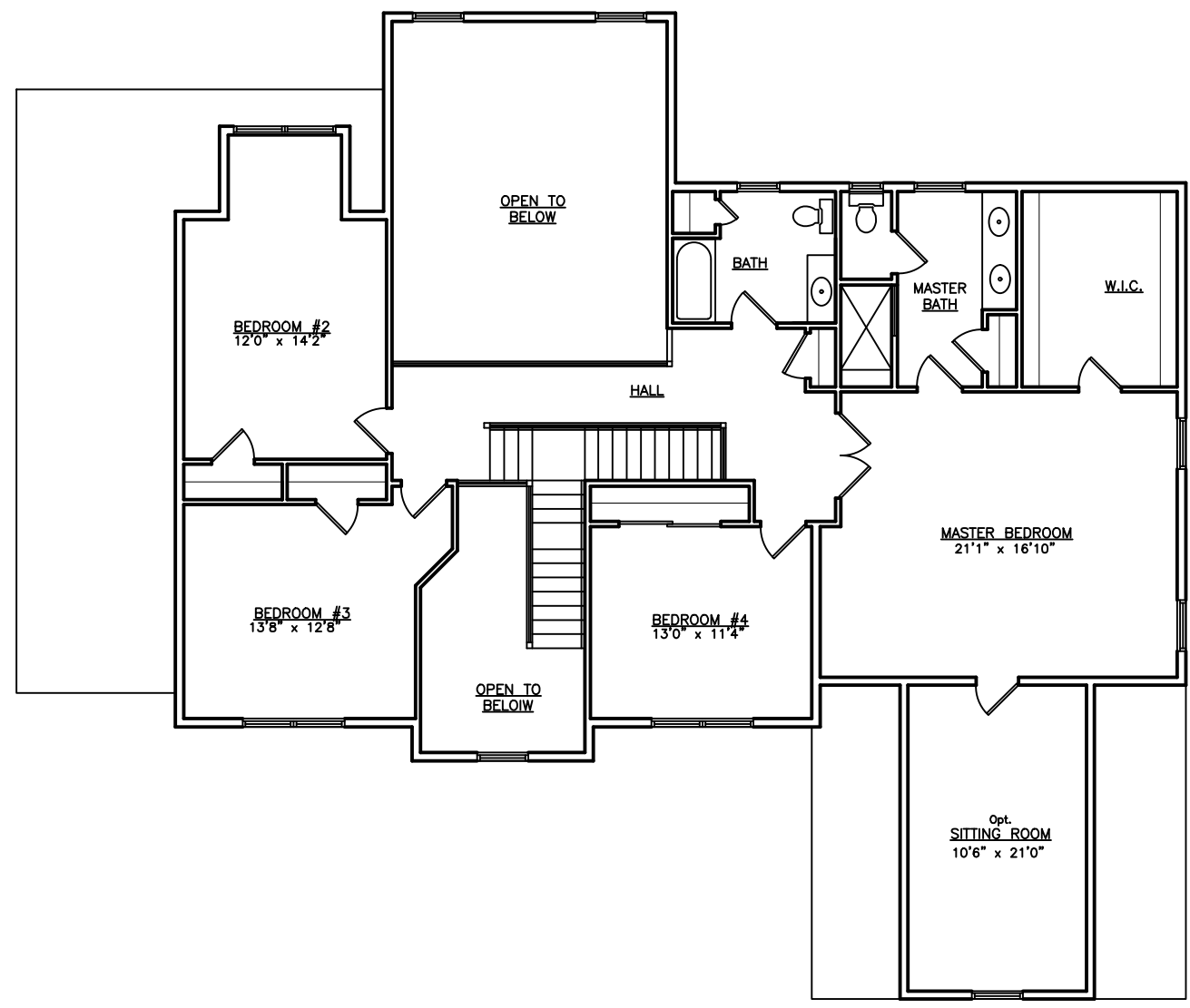
Second floor plan Sq. Ft.: 1732
