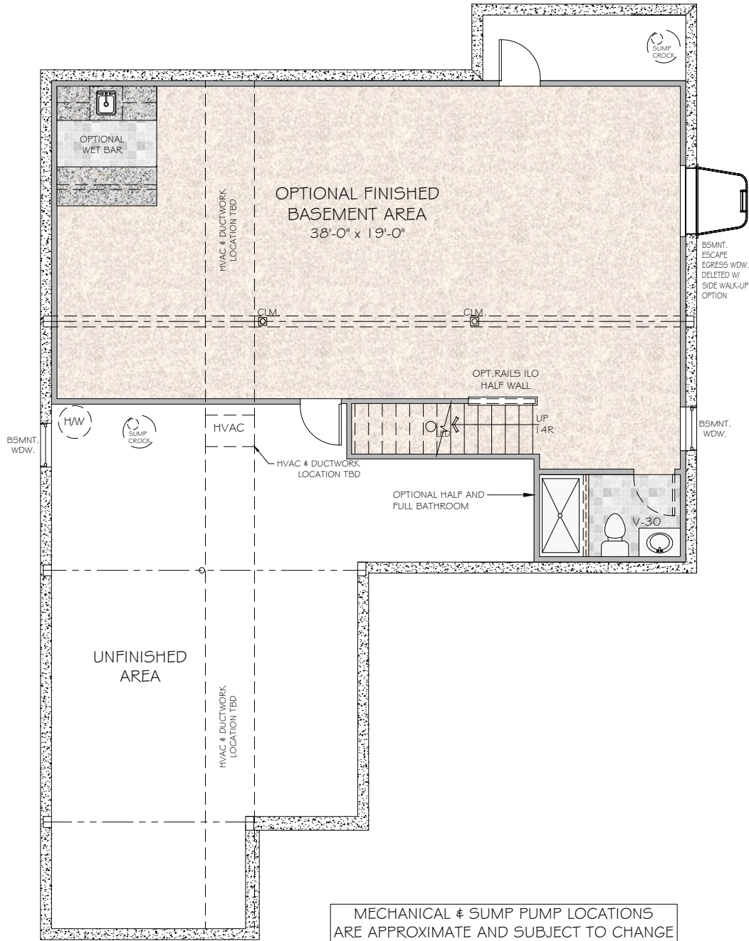
OPTIONAL FINISHED BASEMENT PLAN
