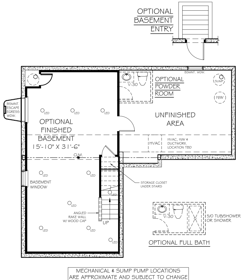
OPTIONAL FINISHED BASEMENT PLAN
