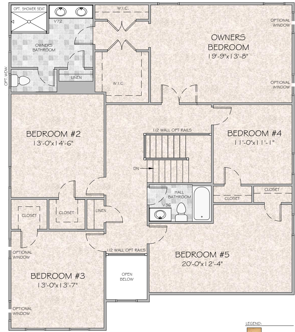
OPT. 5TH BEDROOM
