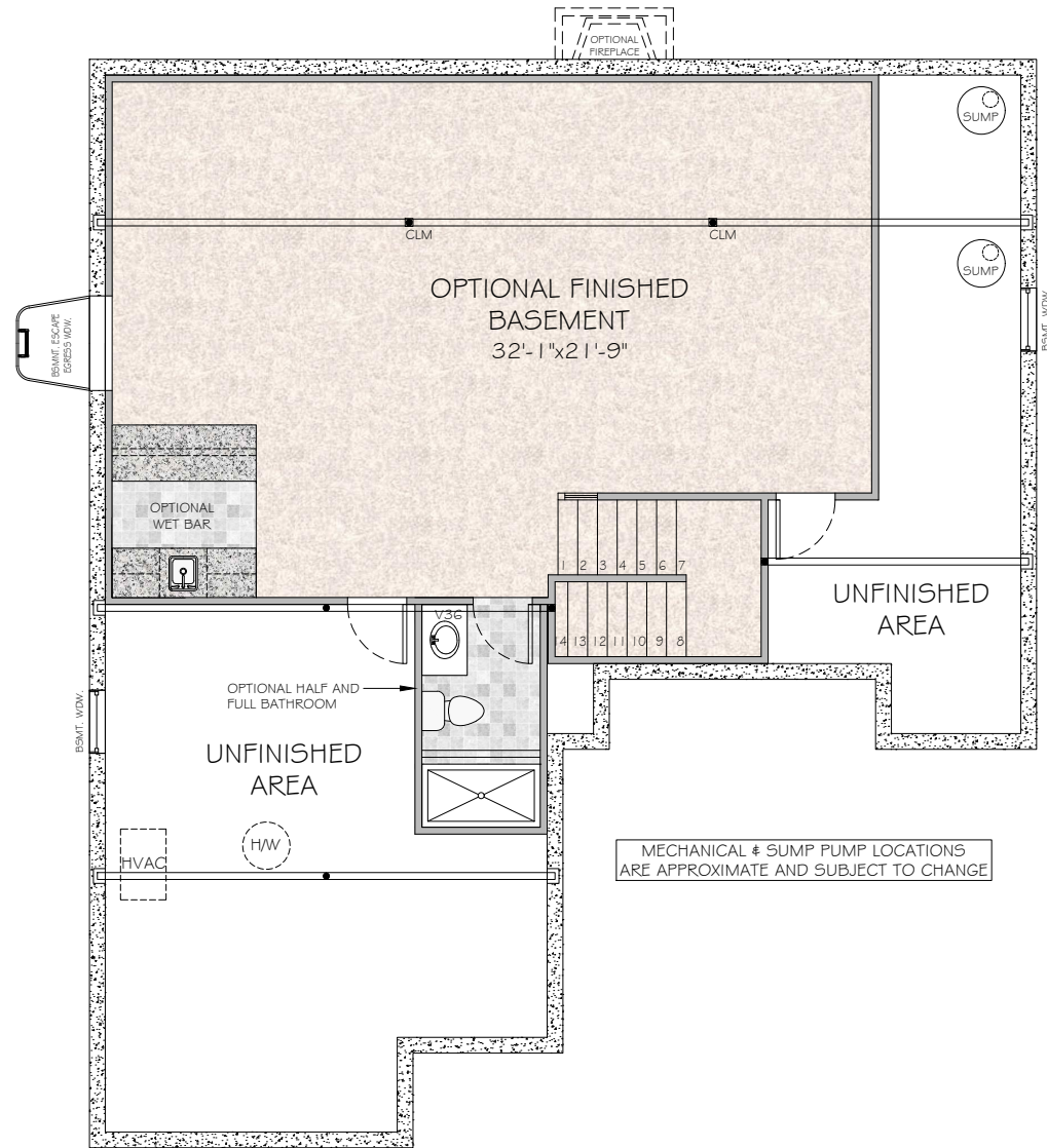
OPTIONAL FINISHED BASEMENT PLAN
