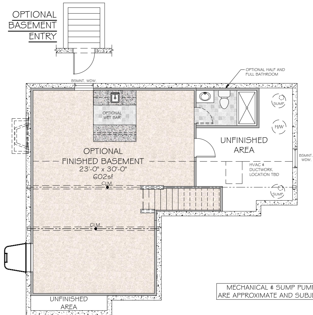
OPTIONAL FINISHED BASEMENT PLAN
