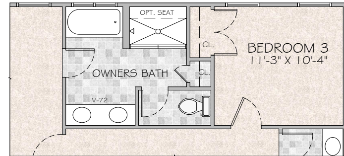
OPT. OWNERS BATHROOM W/OPTIONAL SHOWER SEAT
