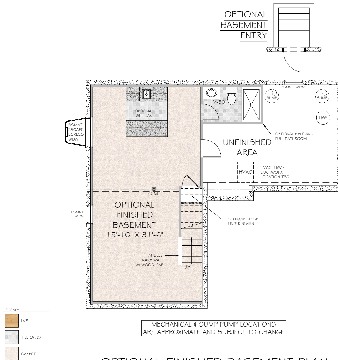
OPTIONAL FINISHED BASEMENT PLAN
