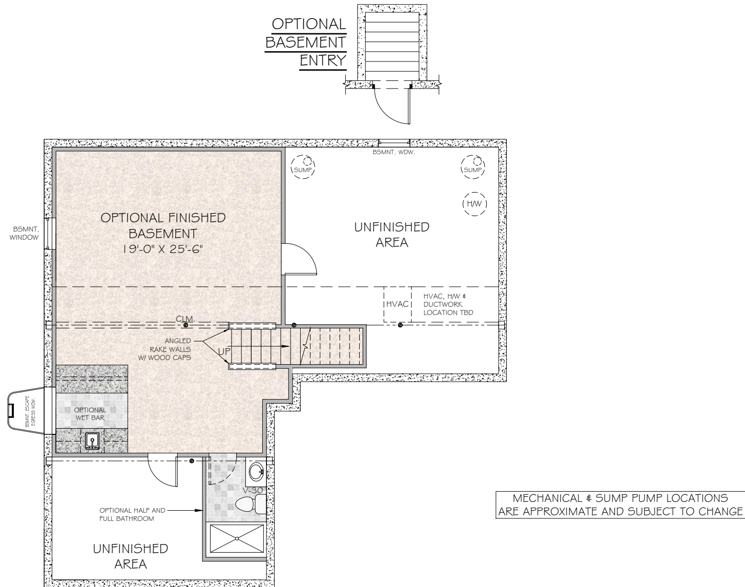
OPTIONAL FINISHED BASEMENT PLAN
