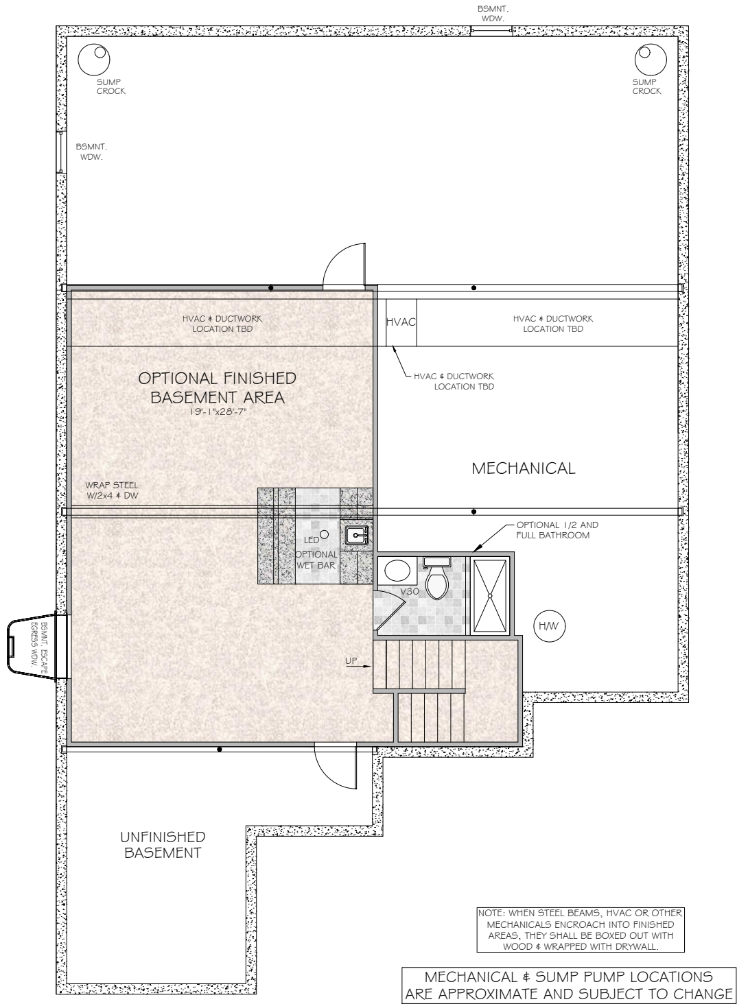
OPTIONAL FINISHED BASEMENT PLAN
