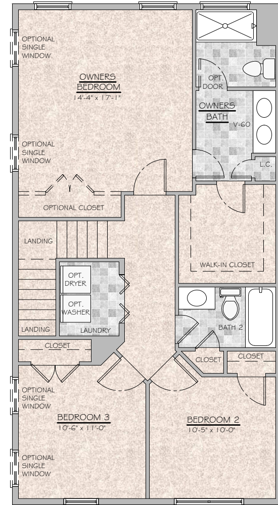
BETHANY SECOND FLOOR
