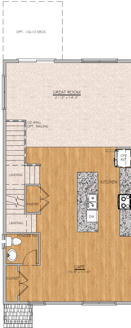
BETHANY FIRST FLOOR
